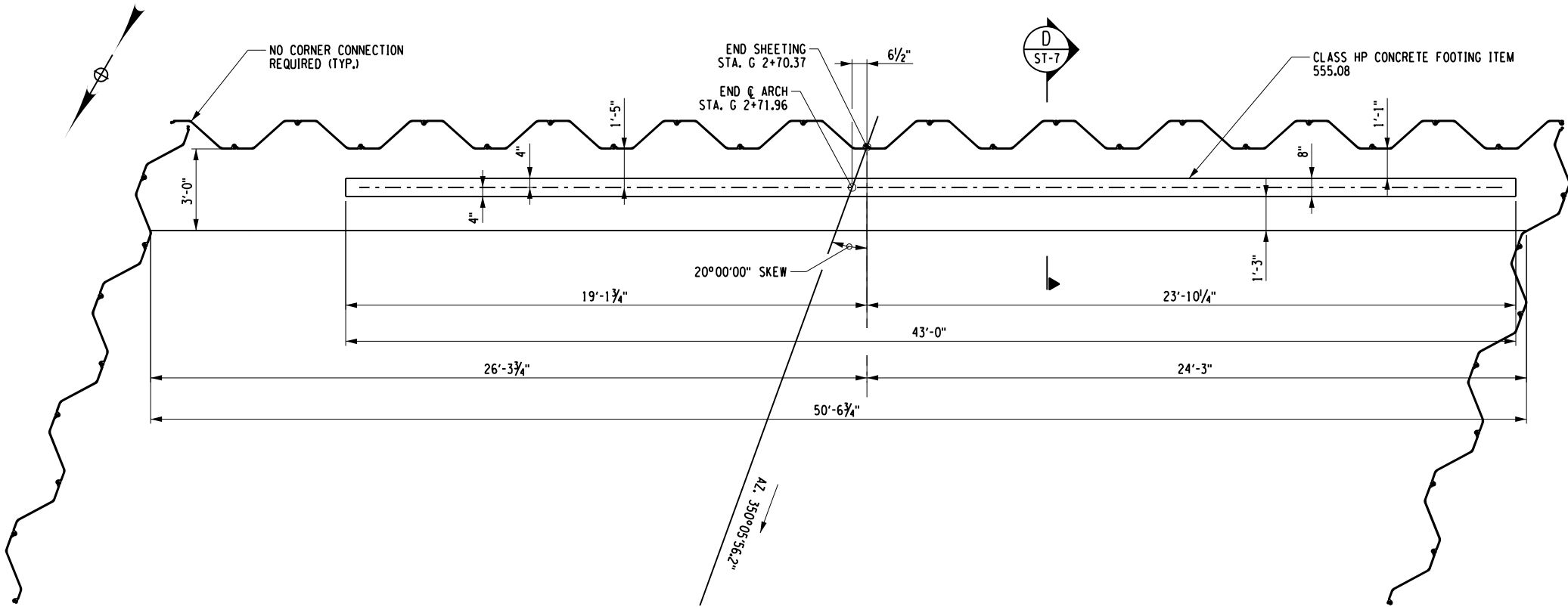
END FOOTING PLAN SCALE: \frac{3}{16}" = 1'-0"
